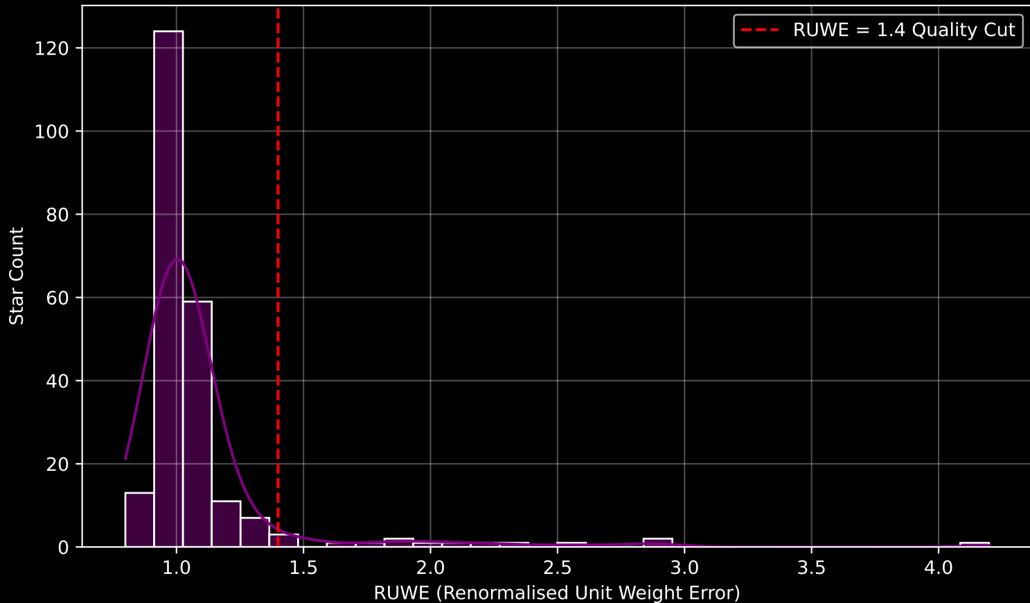
GALAH DR4 Field [8290] RUWE Distribution (n= 229)
