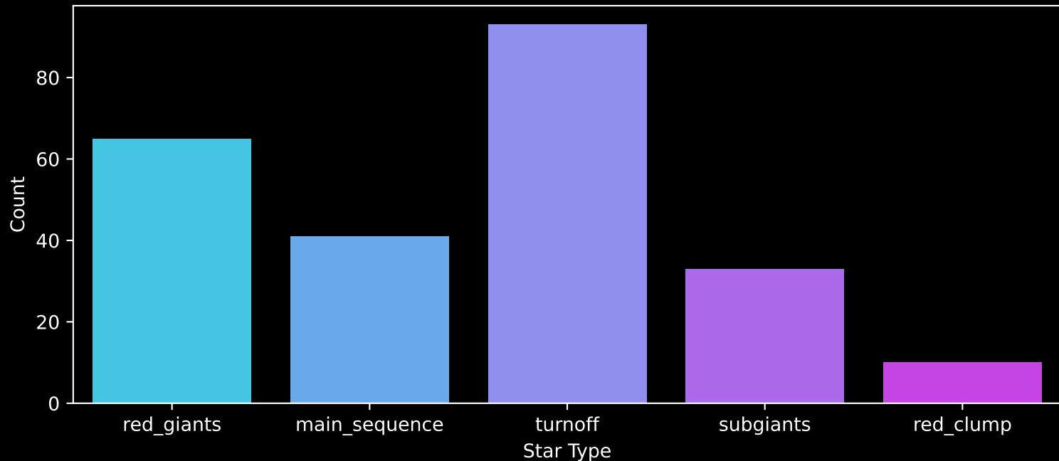
GALAH DR4 Field: [8290] Count plot of Star Type
