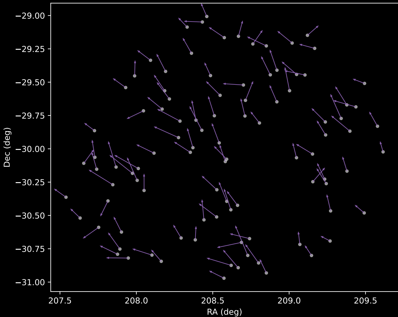
GALAH DR4 Cluster 8 Proper Motion Vectors (n=98)
