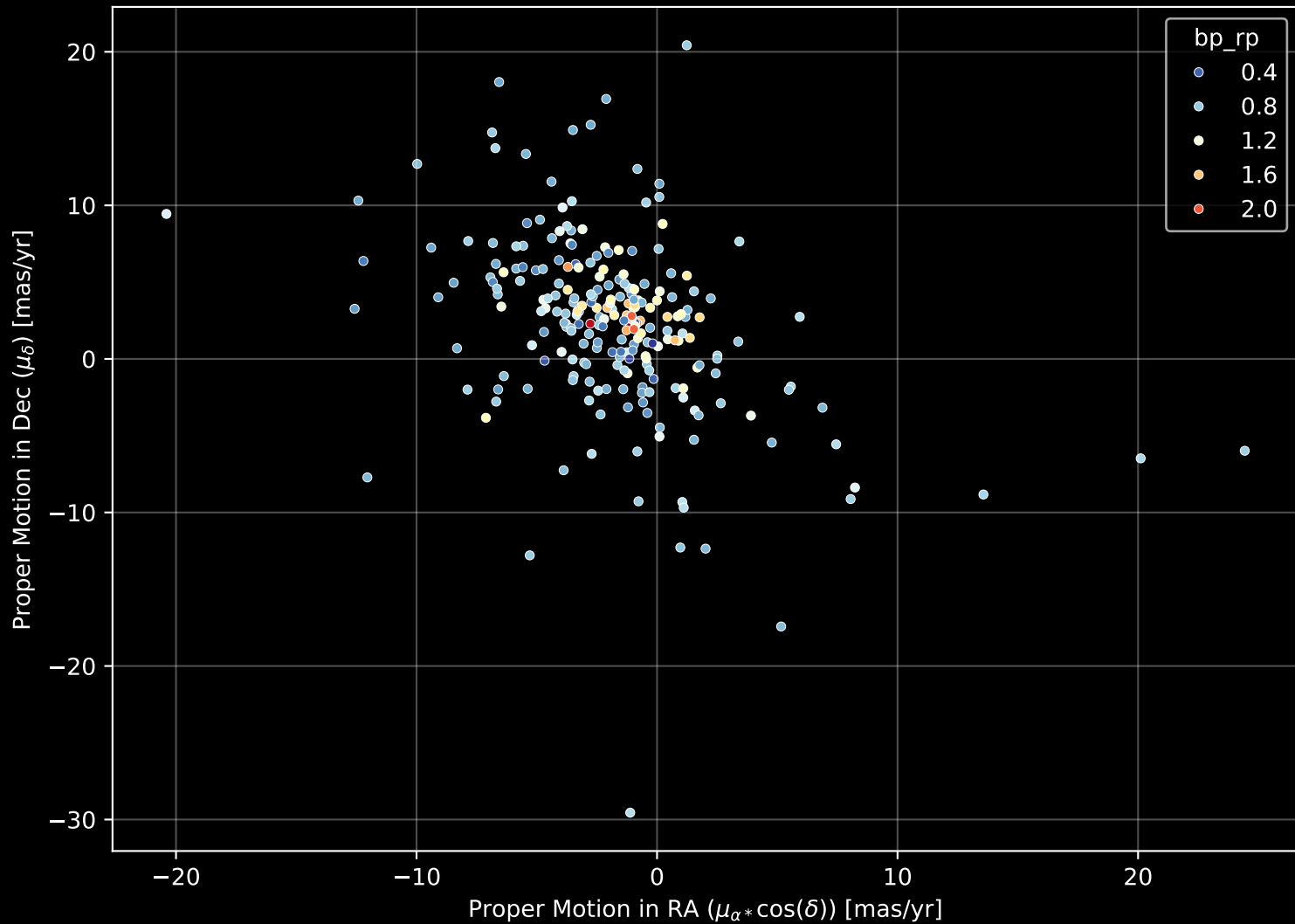
GALAH DR4 Field: [8290] Proper Motion Diagram (n= 242)
